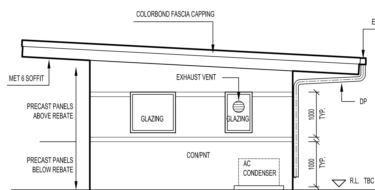
09 NORTH ELEVATION 1:50
