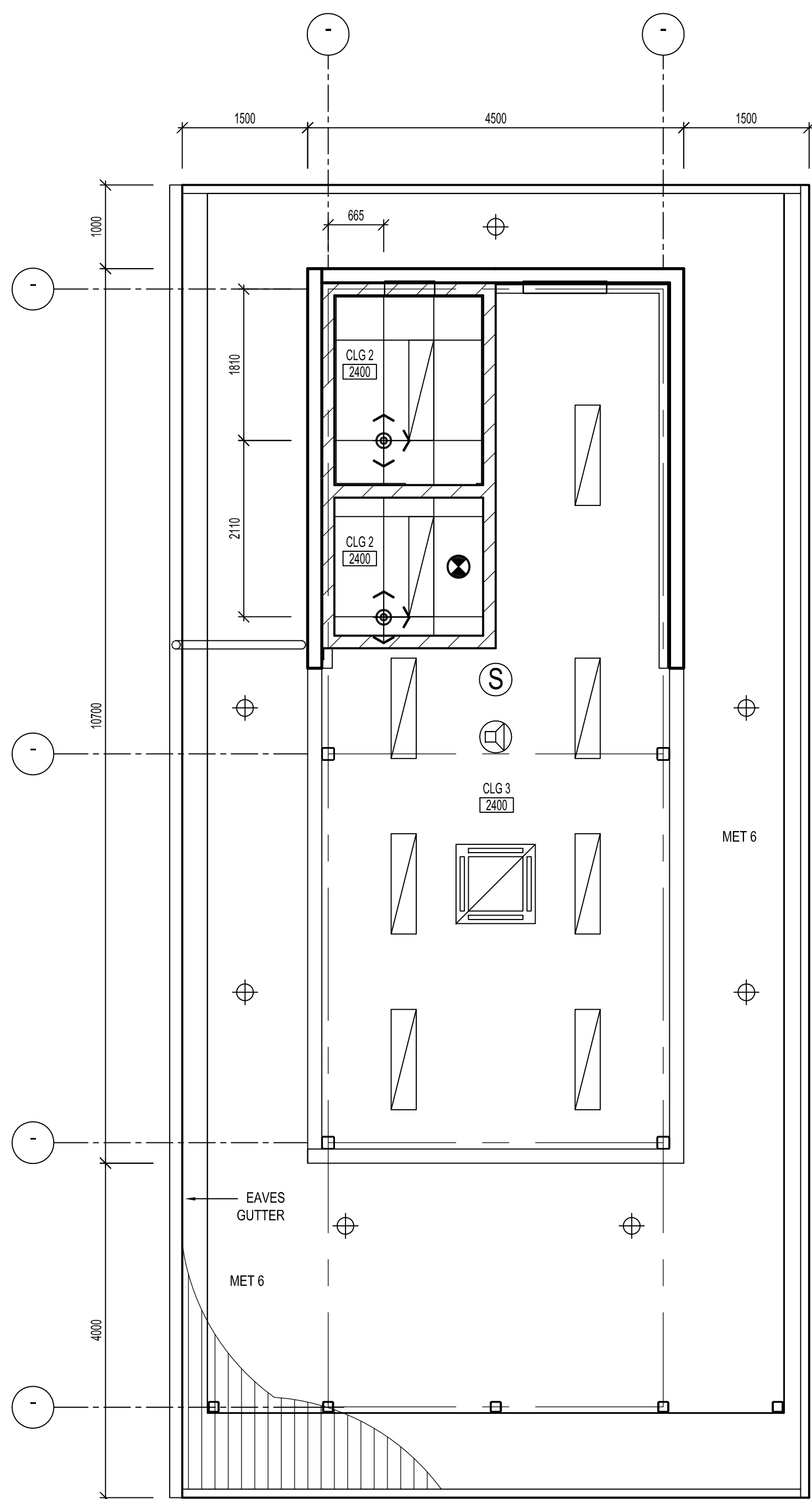
02 REFLECTED CEILING PLAN 1:50
