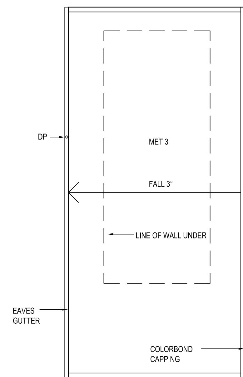
03 ROOF PLAN 1:100
