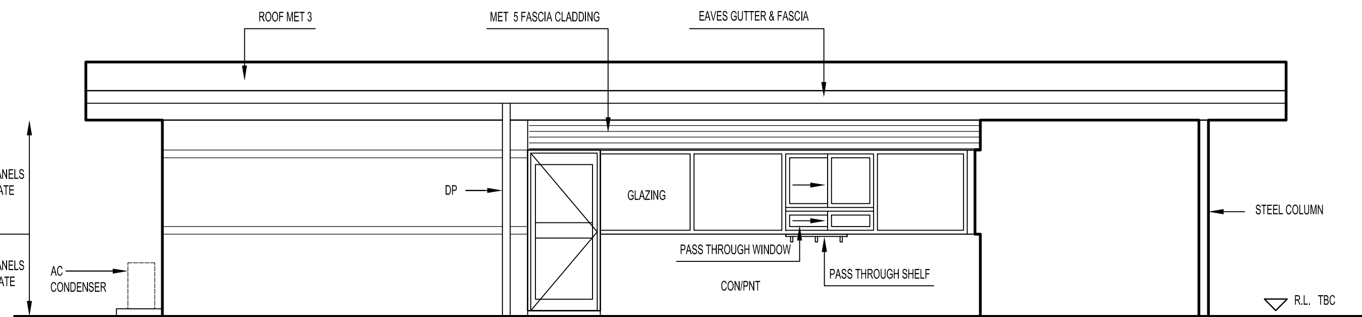
08 WEST ELEVATION 1:50
