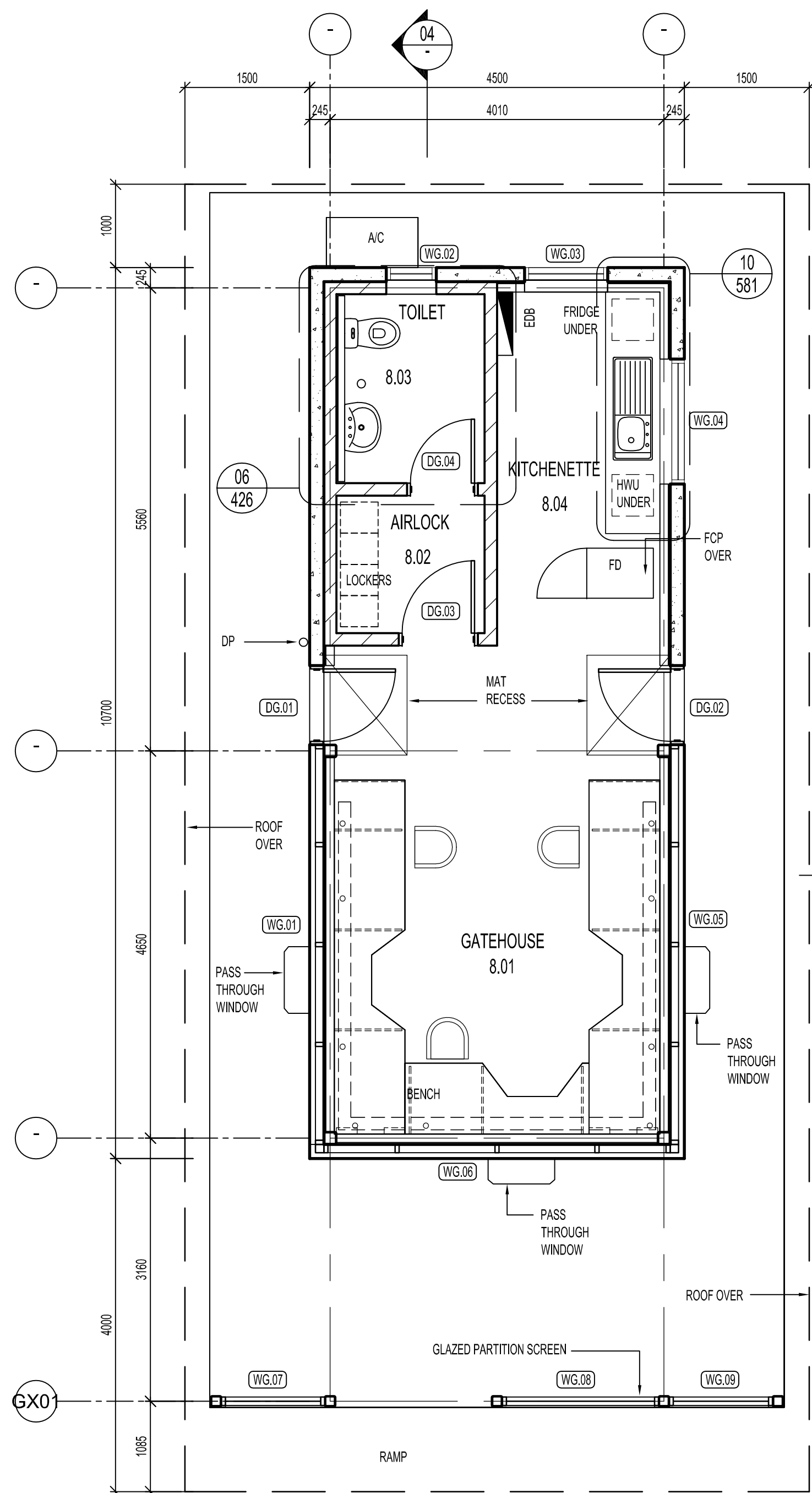
01 FLOOR PLAN 1:50
