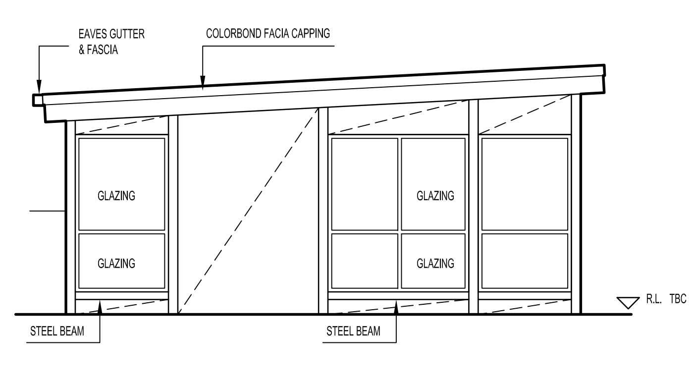
06 SCREEN ELEVATION 1:50
