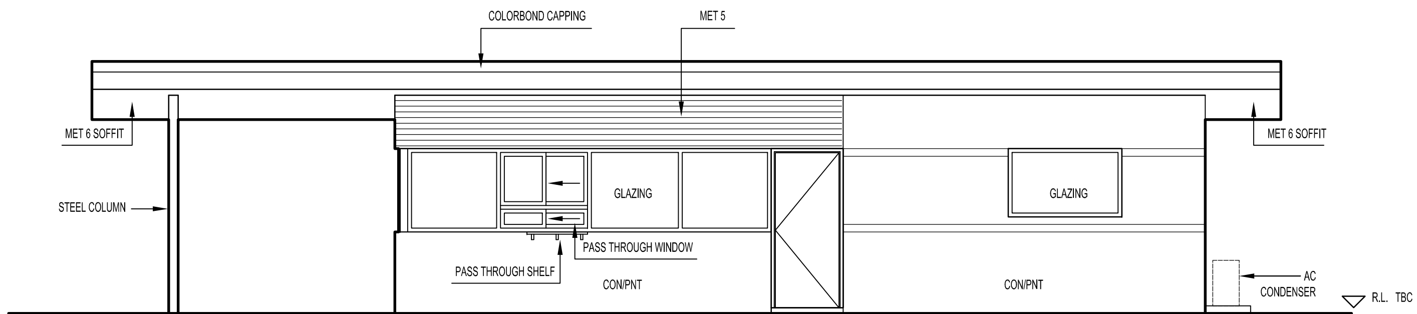
07 EAST ELEVATION 1:50
