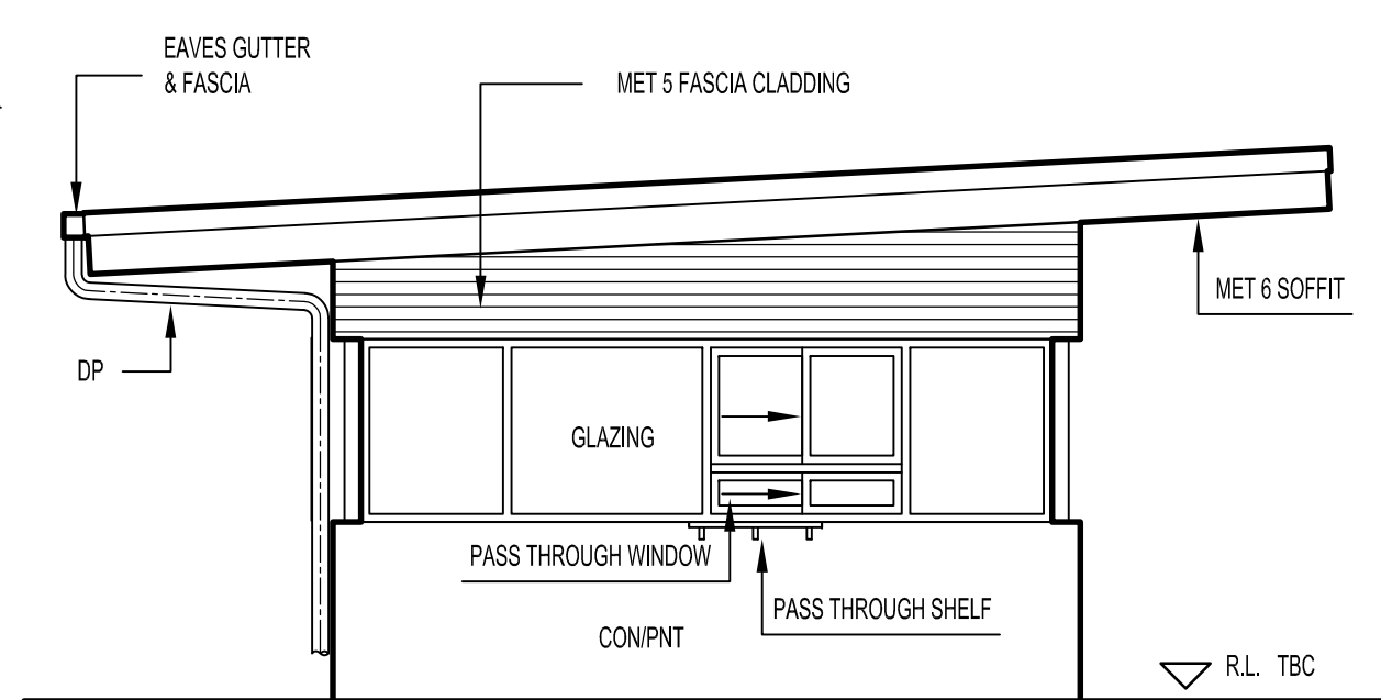
10 SOUTH ELEVATION 1:50
